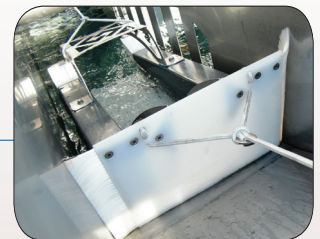
Self-adjusting grease scraper with limited water removal
