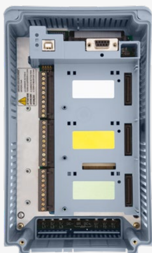
Installation of the PLC module in the CFW11
