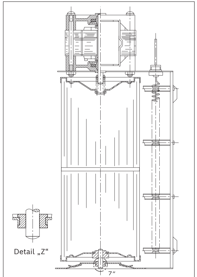
Figure 15: Cross flow fan with plastic plain bearing type R1320-7..
