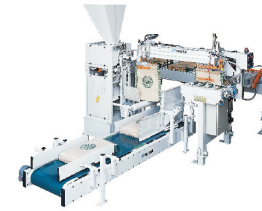
Bagging
