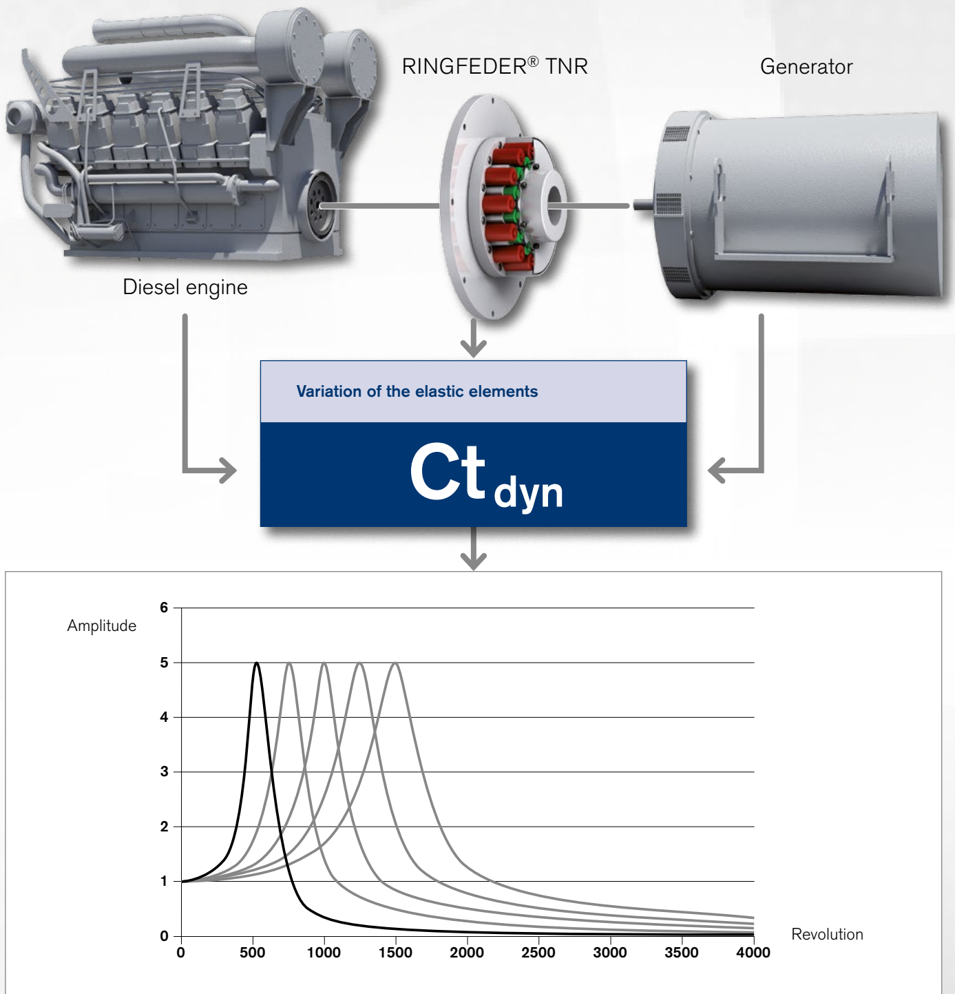
Fig. 2: Interaction of stiffness changes and resonance speeds demonstrated on a diesel engine driven generator
