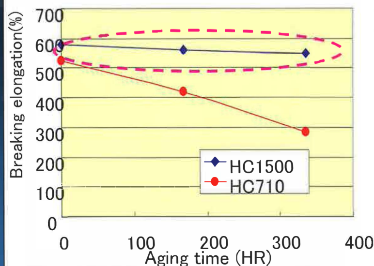
Fig.1 It is possible to put it on 165°C condition making. About the change in breaking expansion EB
