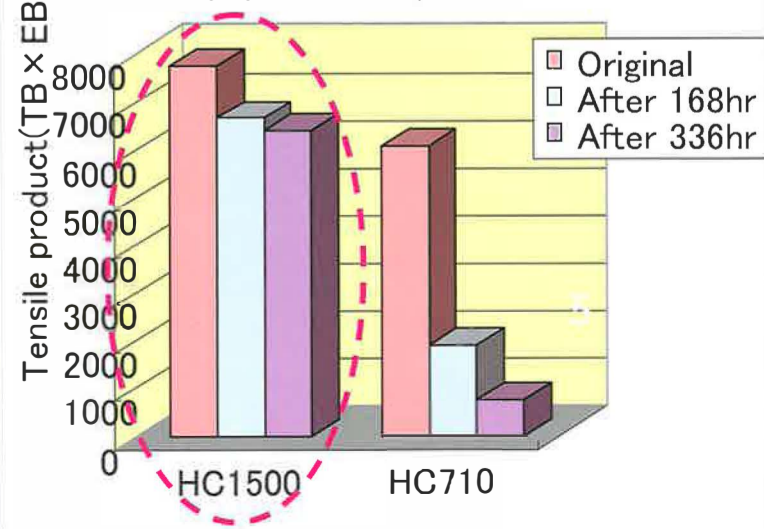
Fig.2 It depends on 165°C aging. About changing the tensile product
