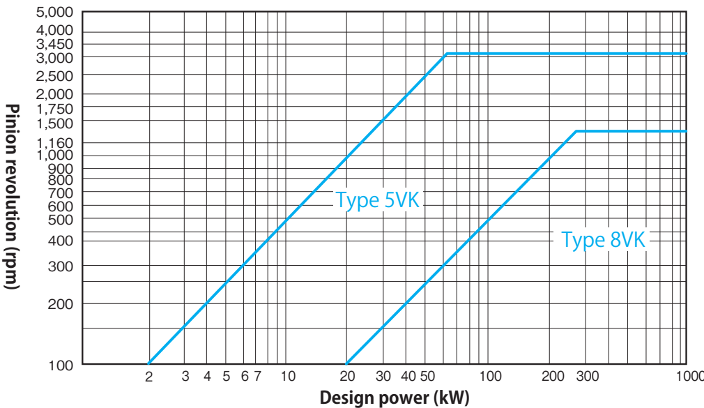
Fig. 1-3 Belt type selection diagram (Power Ace Aramid Combo)
