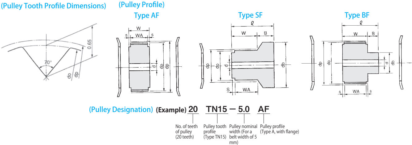
TN15-5.0 (For a belt width of 5 mm)
