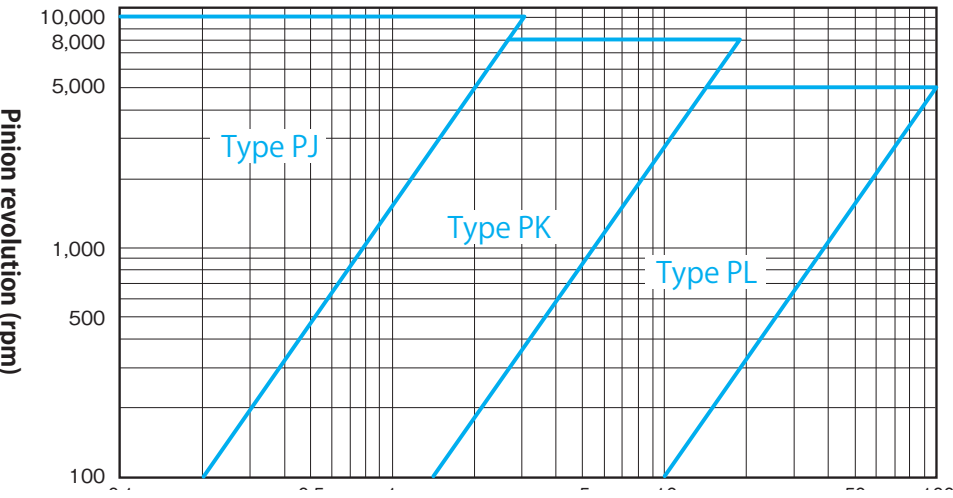
Fig. 1-4 Belt type selection diagram (Rib-Ace 2)
