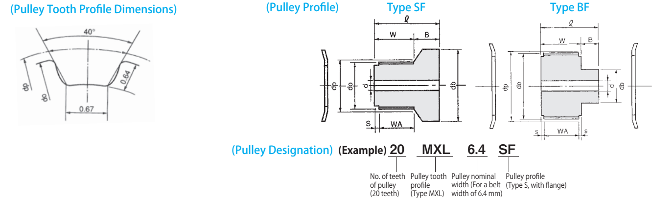
MXL6.4 (For a belt width of 6.4 mm)
