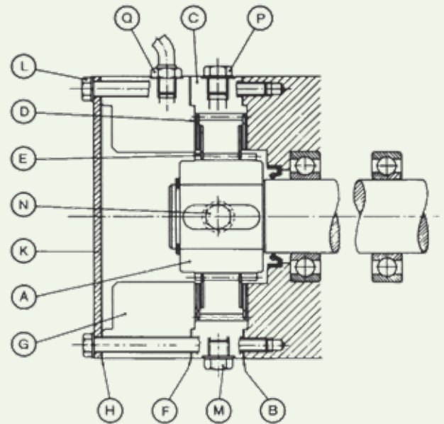
Outboard mounting
