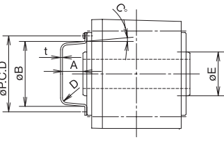
Figure 5.10 Frame Sizes 1200 ~1600
