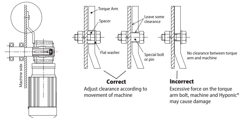
Figure 5.13 Hyponic® Torque Arm Clearance
