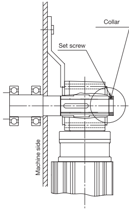
Figure 5.7 Secured by Set Screw and Collar
