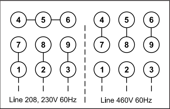
Figure 5.25 EP.NA - WYE
