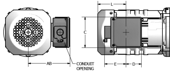
Figure 4.23 Global EP.NA and Outdoor Duty Box
