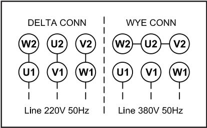
Figure 4.28 DELTA-WYE Diagram
