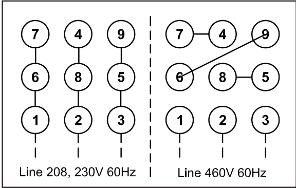
Figure 5.26 EP.NA - DELTA
