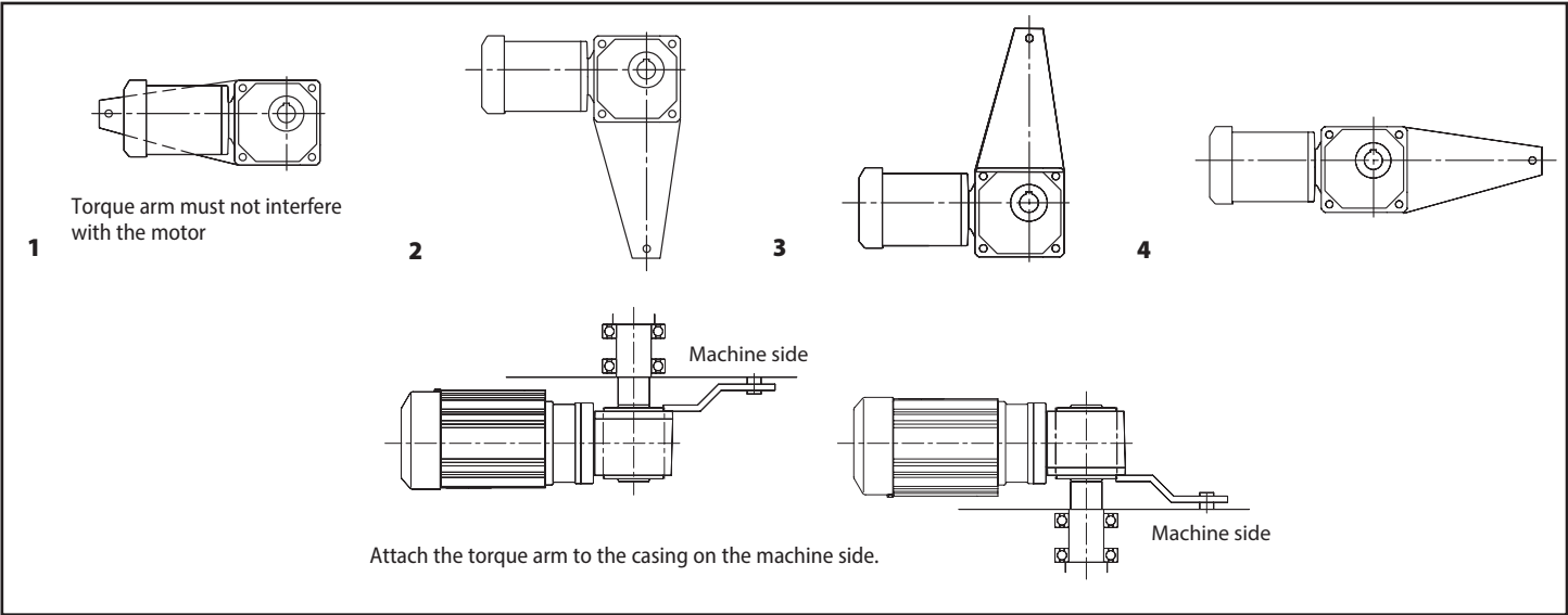
Figure 5.12 Hyponic® Torque Arm Mounting Examples
