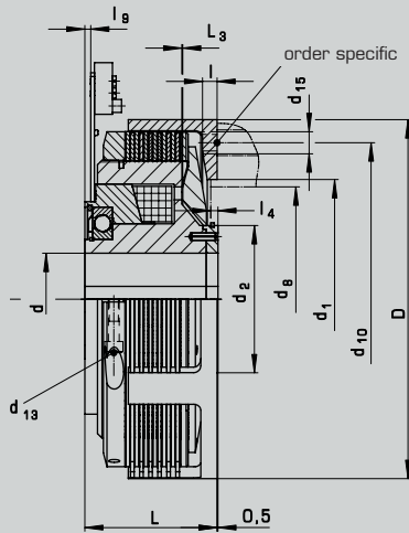
Typ 521...1 with normal drive ring
