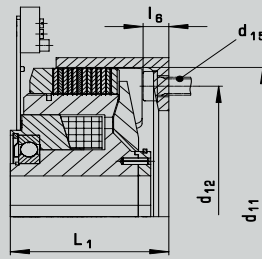
Typ 521...2 with long drive ring
