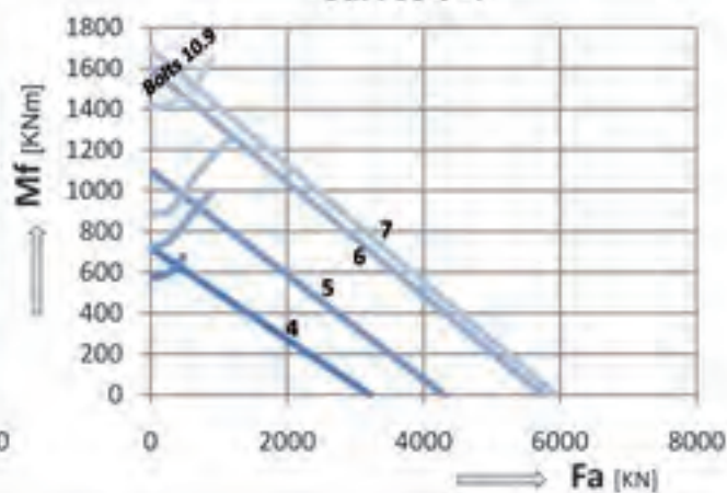
Curves 4-7
