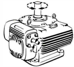
VD - shaft handing "R/LX"
